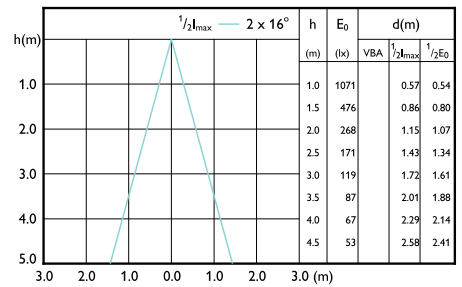
Downlight RS061B 827 PSR WH LILO-LBP
