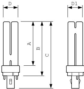
MASTER PL-C 18W/830 /2P ICT/5X10BOX
