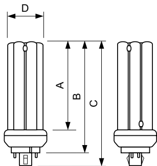
MASTER PL-T TOP 26W/830/4P 1CT/5X10BOX
