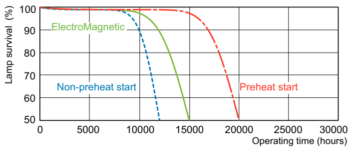
Life Expectancy Diagram - TL-D 30W/827 1PP/10
