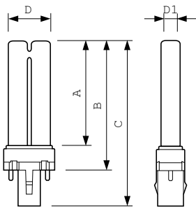
PL-S 11W/827/2P LM
