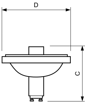
MASTERColour CDM-R111 Elite CDM-R111 Elite 35W/930 GX8.5 24D
