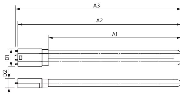
CorePro LED PLL HF 16.5W 865 4P 2G11
