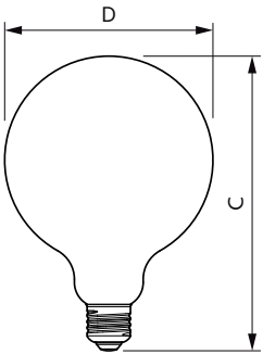
G120 50W 630lm 2700K E27 D Crown Mirror
