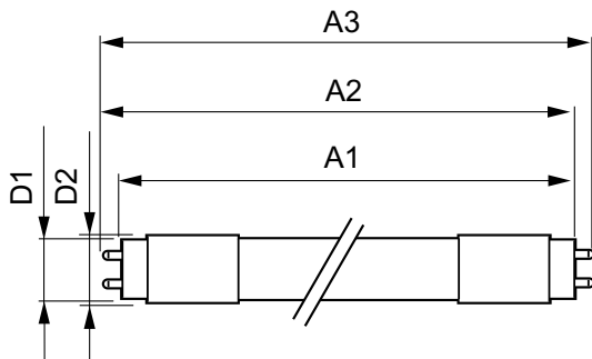
TLED 4ft 230V 16.5-32W 2500lm 6500K G13
