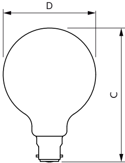
Bulb G93 EU 6-60W 810lm WG B22 CL
